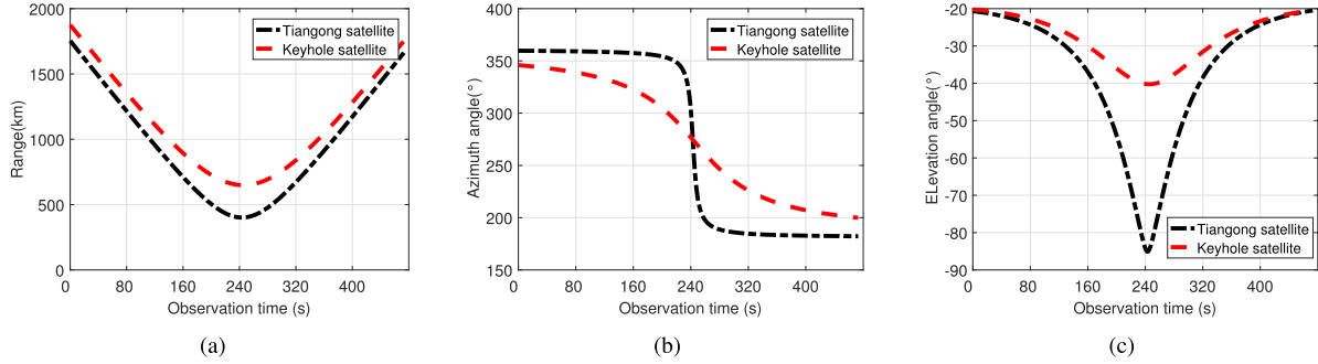
Fig. 15. (a) Distance, (b) azimuth angle, and (c) elevation angle of the satellite in orbit acquired using STK software.
