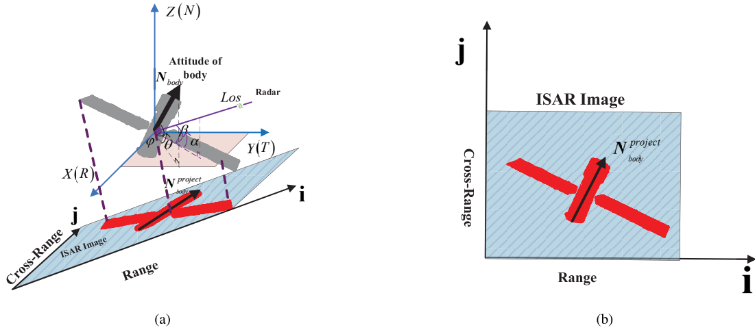
Fig. 2. ISAR imaging of satellite. (a) ISAR imaging geometry in local orbit frame and the projection process of ISAR imaging. (b) ISAR image.
