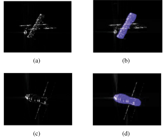
Fig. 3. ISAR image segmentation examples of satellite targets (the first row shows the KH satellite images; the second row shows the TG satellite images). (a) and (c) Original ISAR images. (b) and (d) Labeled ISAR images.
