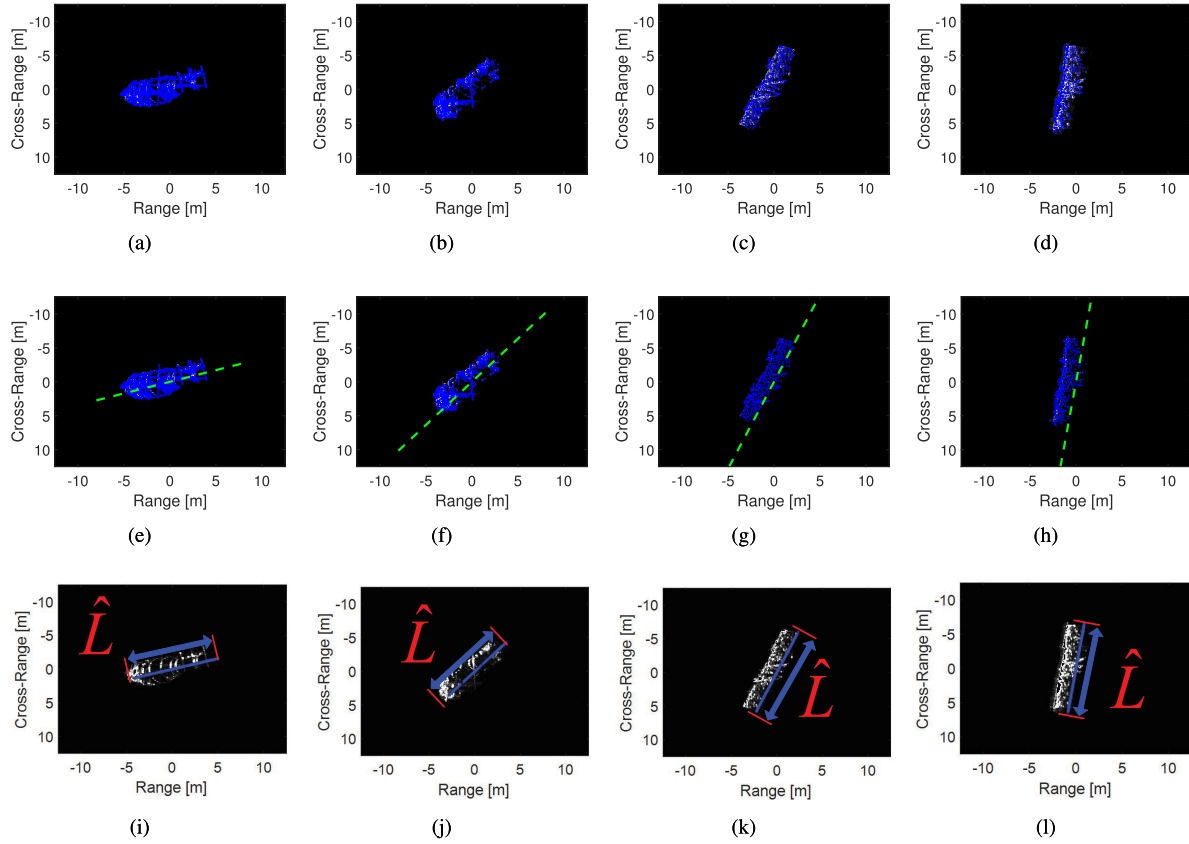
Fig. 12. Feature extraction from the segmented satellite's capsules. (a)–(d) Obtained scatterers of the satellite's capsules. (e)–(h) 2-D orientation of the satellite's capsules. (i)–(l) Projected capsule lengths of the satellite.
