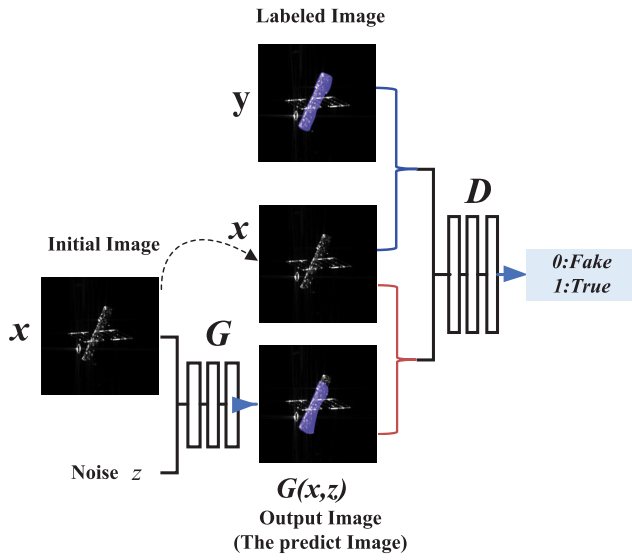
Fig. 4. Training process of Pix2pixGAN.
