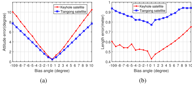
Fig. 14. Variation of attitude and length estimation errors with bias error of PCA feature extraction. (a) Variation of attitude estimation error with bias. (b) Variation of length estimation error with bias.
