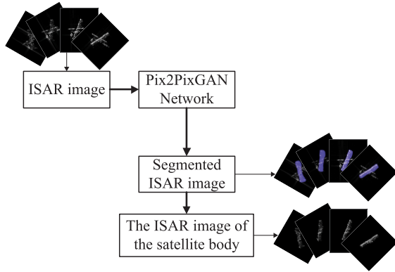
Fig. 5. Flowchart of the proposed ISAR image segmentation method.
