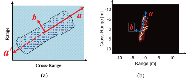
Fig. 6. Geometry of scattering centers distribution and its principal components. (a) Satellite's capsule and its principal component. (b) Simulated satellite's capsule.
