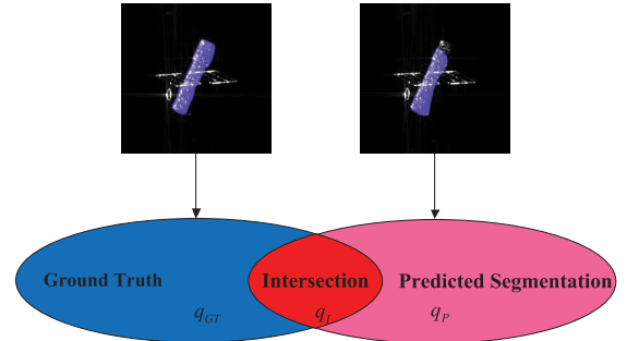
Fig. 10. MIoU interpretation of ISAR image segmentation. The left ISAR image is the ground truth, and the right ISAR image is the segmented image predicted by segmentation algorithms.
