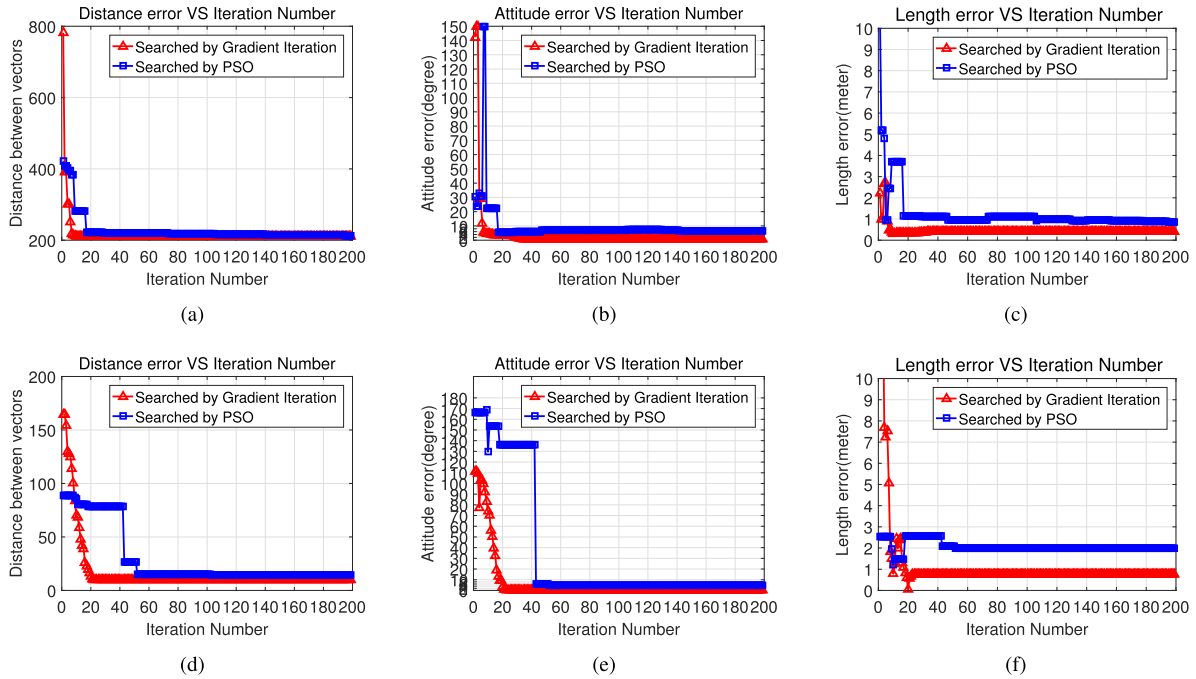
Fig. 13. Optimization functions and the variation of size and attitude estimation errors with the number of iterations. (a) and (d) Variation curves of optimization functions with the number of iterations for KH and TG satellites. (b) and (e) Variation curves of attitude estimation errors with the number of iterations for KH and TG satellites. (c) and (f) Variation curves of size errors with the number of iterations for KH and TG satellites.
