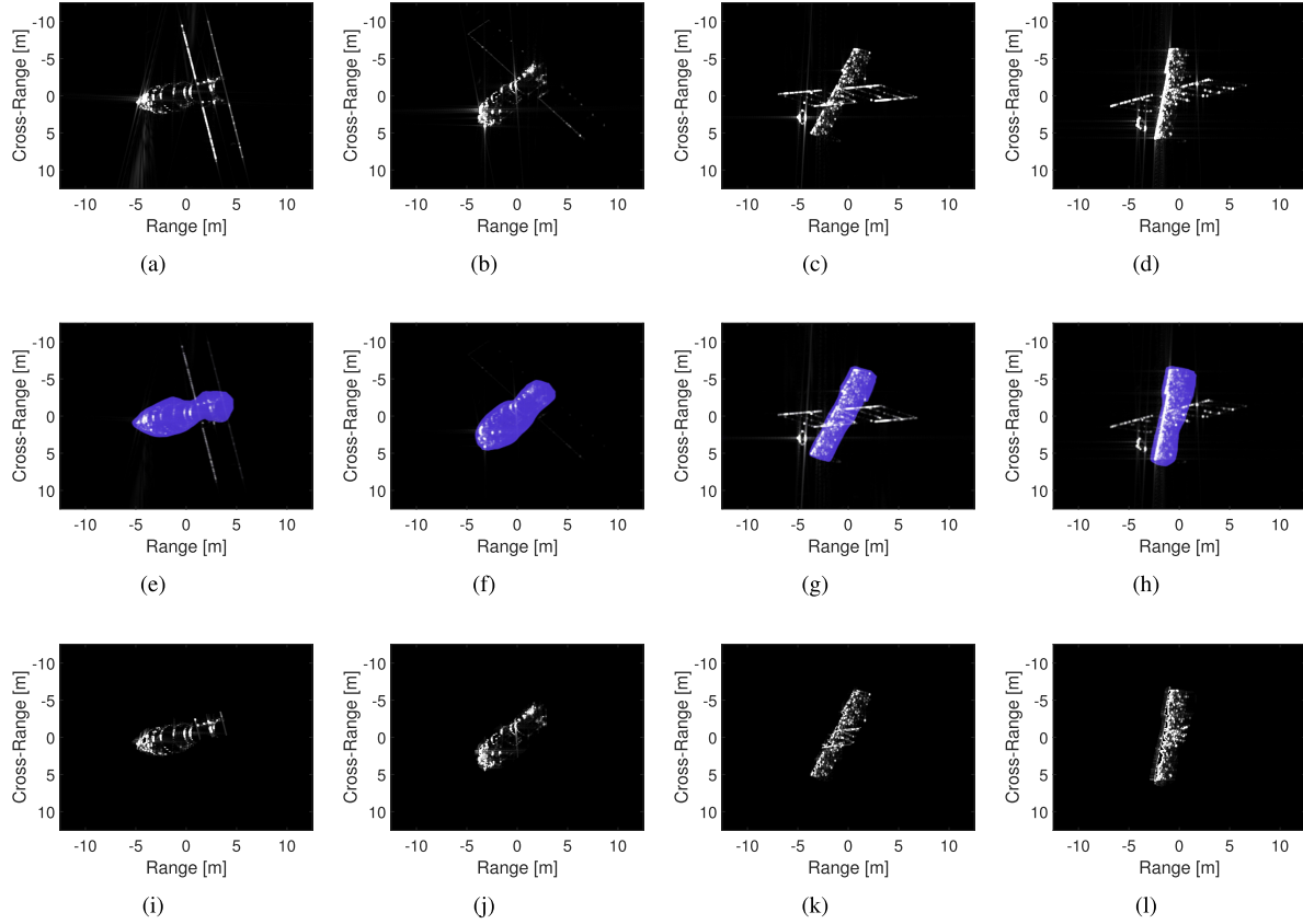
Fig. 11. Some examples of the segmentation outputs. (a)–(d) Initial ISAR images. (e)–(h) Output of the Pix2pixGAN network (labeled images). (i)–(l) Segmented satellite's capsule. (a), (e), and (i) 18th frame of TG. (b), (f), and (j) 42nd frame of TG. (c), (g), and (k) 25th frame of KH. (d), (h), and (l) 35th frame of KH.
