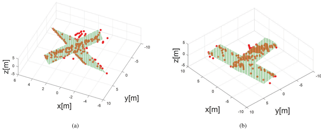
Fig. 17. Reconstruct results of these two satellite. (a) 3-D scatterers of KH. (b) 3-D scatterers of TG.
