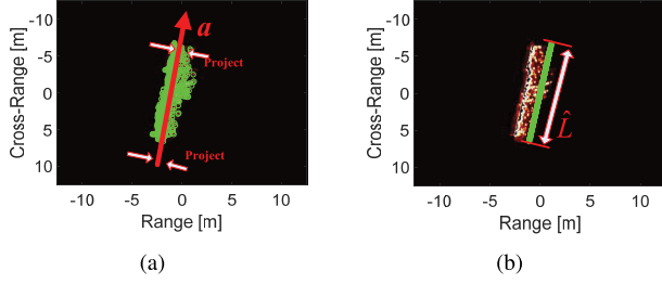
Fig. 7. Extracted length of the satellite's capsule. (a) Satellite's capsule and extracted scatterers' centers. (b) Projected length of the satellite's capsule.
