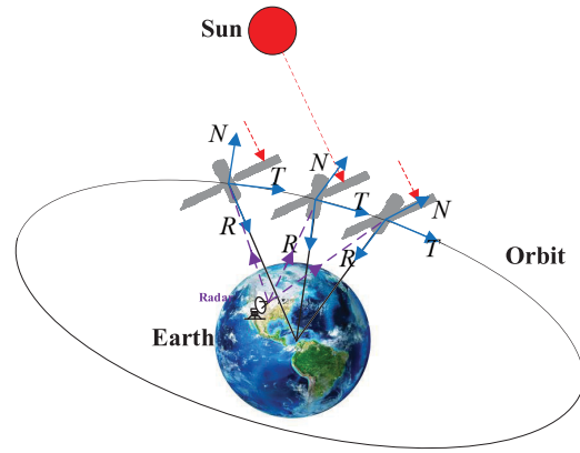
Fig. 1. Observation geometry of satellite in orbit.
