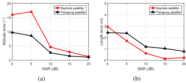
Fig. 16. Curves of attitude and size estimation errors with SNR. (a) Variation curve of attitude error with SNR. (b) Variation curve of size error with SNR.
