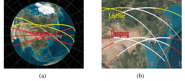
Fig. 9. Orbits of TG and KH satellites simulated by STK. (a) Trajectory of these satellites that circle the Earth three times. (b) Trajectory segments observable by radar (white).
