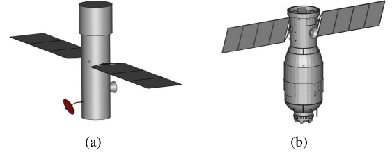
Fig. 8. CAD models of two satellite targets. (a) CAD model of the KH satellite. (b) CAD model of the TG satellite.
